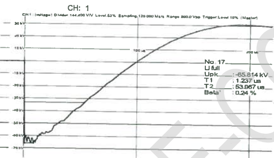
No. 17 Li full Upk: -65.814 kV T1: 1.237 µs T2: 53.967 µs Beta': 0.24 %
