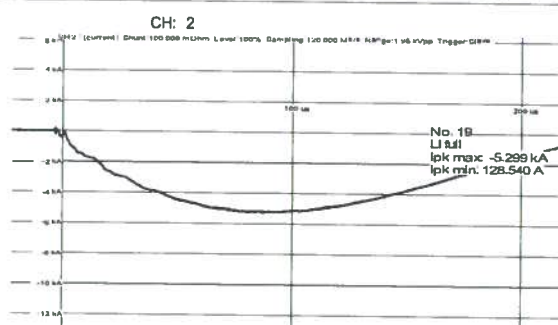
No. 19 LI full Ip max: -5.299 kA Ip min: 128.540 A
