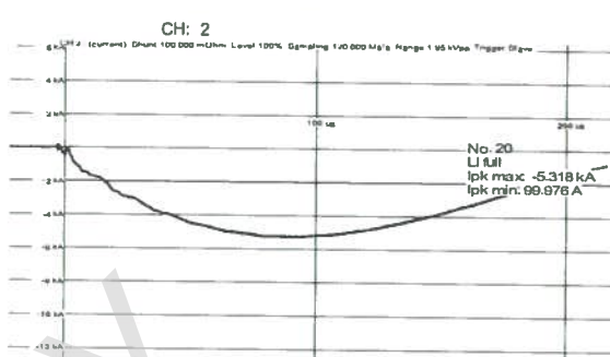
No. 20 LI full Ip max: -5.318 kA Ip min: 99.976 A
