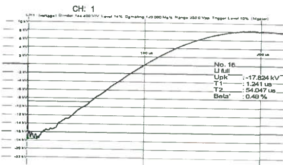
No. 16 Li full Upk: -17.824 kV T1: 1.241 µs T2: 54.047 µs Beta': 0.49 %
