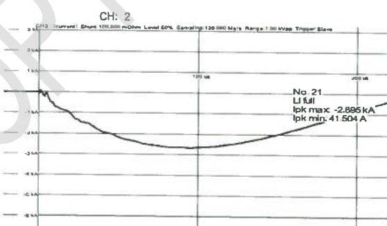
No. 21 LI full Ip max: -2.695 kA Ip min: 41.504 A
