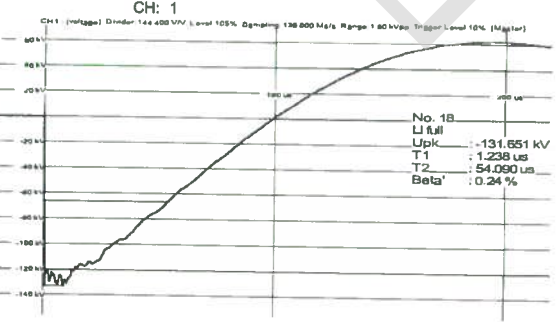
No. 18 Li full Upk: -131.651 kV T1: 1.238 µs T2: 54.090 µs Beta': 0.24 %
