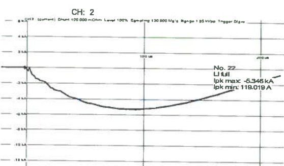
No. 22 LI full Ip max: -5.346 kA Ip min: 119.019 A
