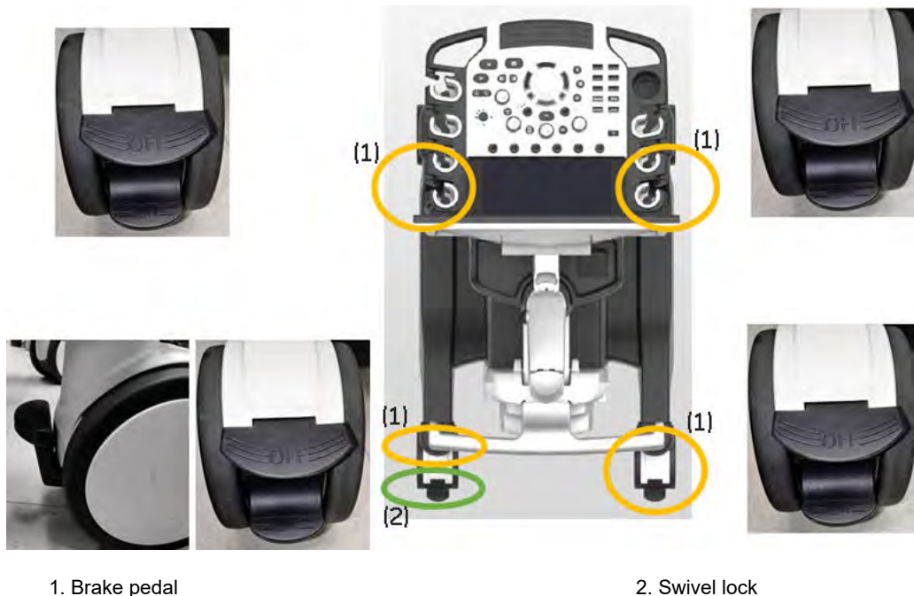
Figure 3-52 Wheel lock and Swivel lock
