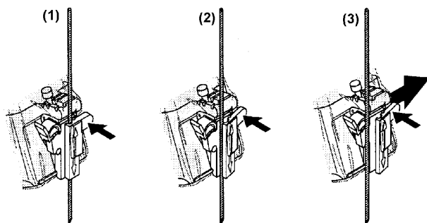
Figure 11-41 Release the needle from assembly
