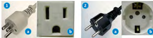
Figure 3-14 Example Plug and Outlet Configurations
