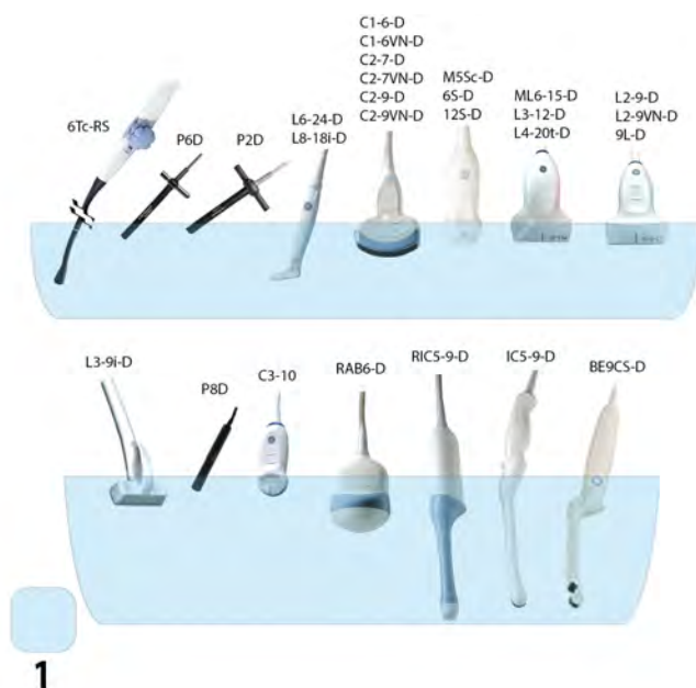
Figure 11-14 Probe Immersion Levels, 1 = Fluid Level
