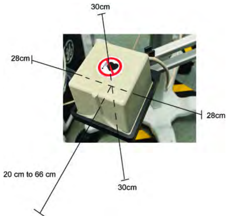
Figure 13-138 Magnetic Field Range from the Transmitter
