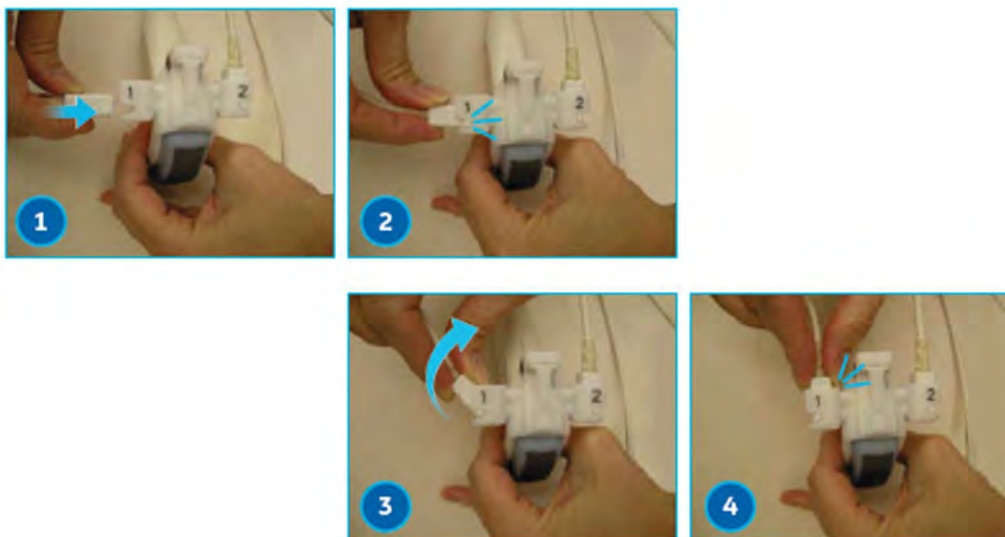
Figure 13-135 Set up the position sensor
