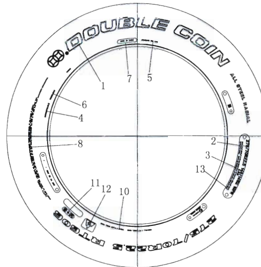
UPPER MOLD
