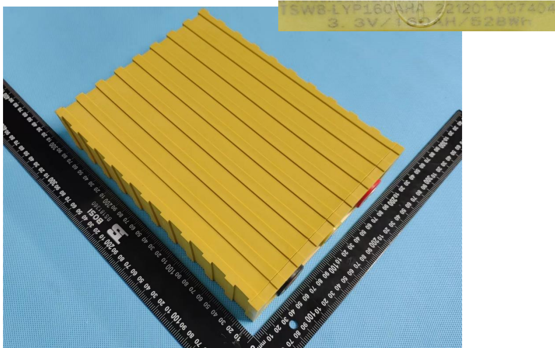
Photo 1 电池正面 Front view of Cell
